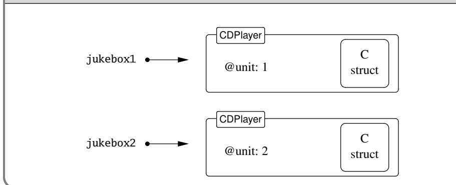
Figure 29.1. Wrapping Objects Around C Data Types
