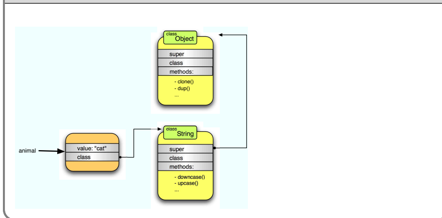
Figure 24.1. Object Model for a Basic Class
