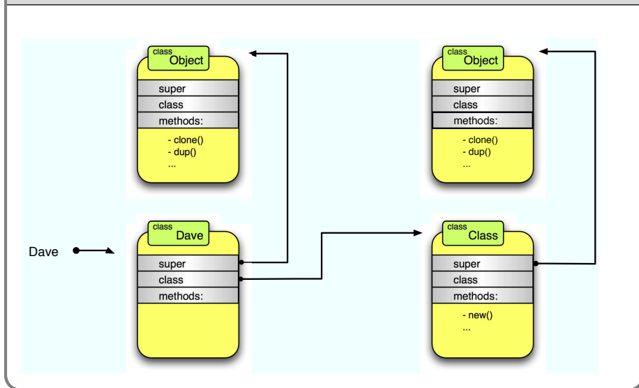
Figure 24.3. Basic Class Definition
